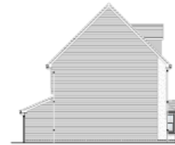
Left Elevation
