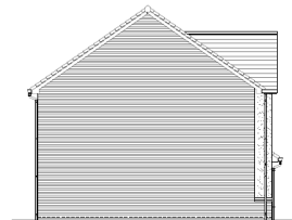
Left Elevation
